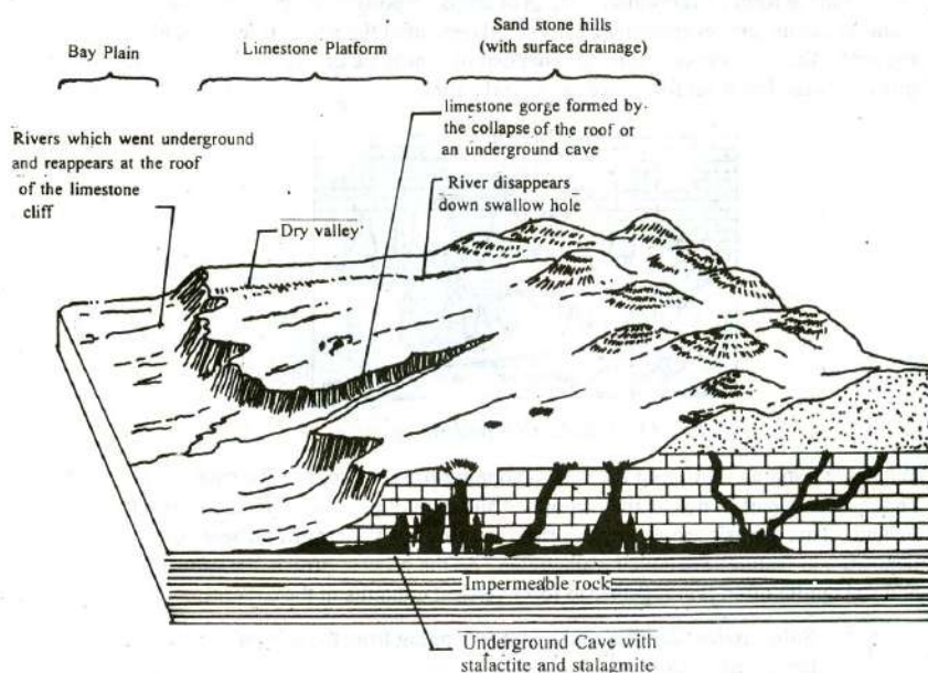
Fig. 5.14 : Limestone Landscape
